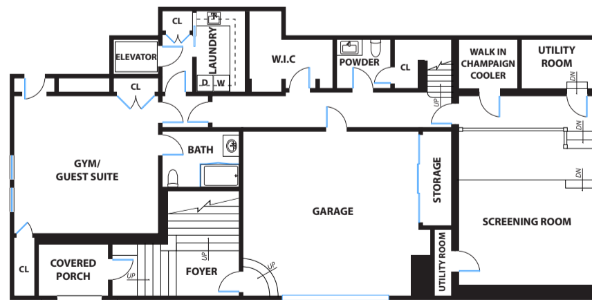
BASEMENT/ GARAGE LEVEL
